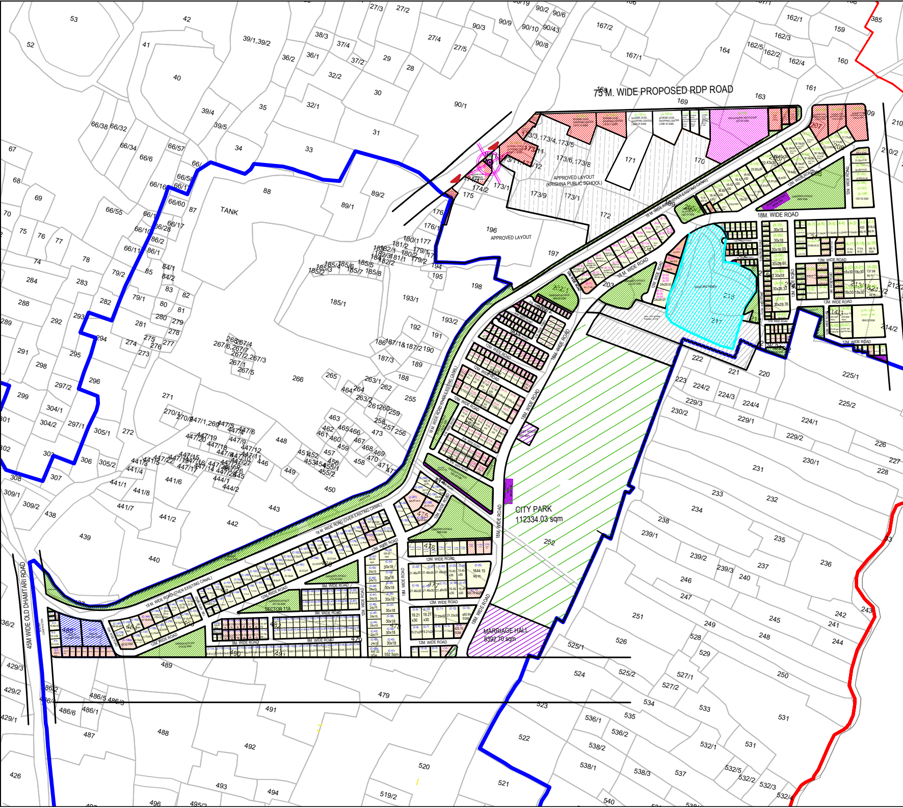
LAYOUT PLAN
